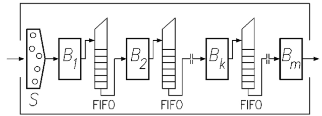
Fig. 2 Permutation flow shop system, where FIFO is the First In First Out
